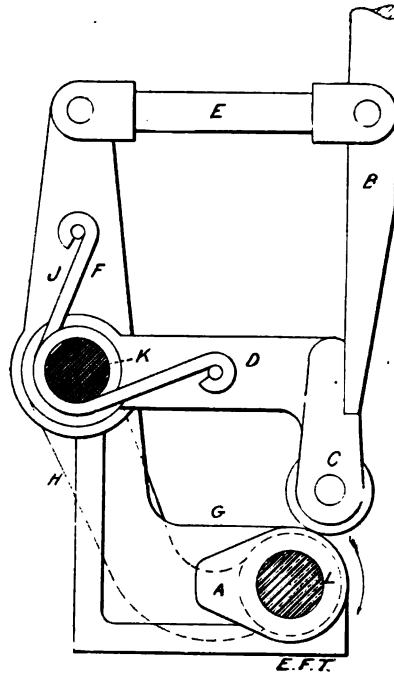
FIG. 396.—Governor Mechanism of the later Daimler Motors. As shown in this cut, the cam, A, bearing upon the roller, C, lifts the arm, D, pivoted at K, and held in position by a spring, J. By lifting arm, D, it also lifts pushrod, B, which opens the exhaust valve. When, however, the speed of the motor has increased beyond the predetermined limit a sleeve of varying diameter, sliding on the same shaft, L, to which the cam, A, is fixed, is moved so that the larger diameter is brought to bear against the downward extension, H, of the arm, F, thus causing F to incline on the pivot, K, toward the cylinder (at the right as in the cut), hence pushing rod, B, by link, E, out of range of arm, D, as it is moved upward by impulse from cam, A. In this case the exhaust valve is not opened and the products of combustion being retained in the cylinder, there is no feeding of fresh fuel gas.
